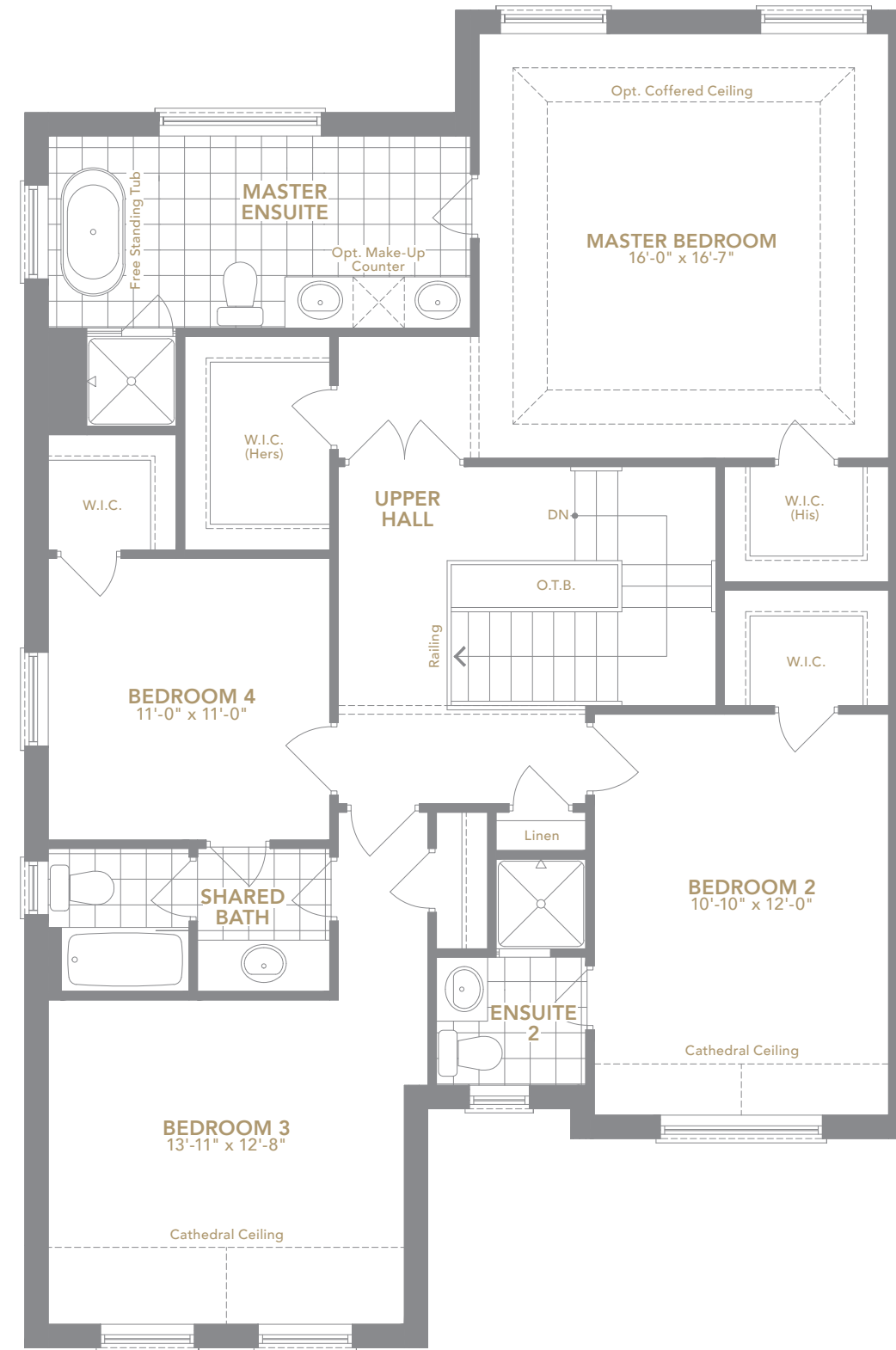
ELEVATION A | SECOND FLOOR | 4 BEDROOM
