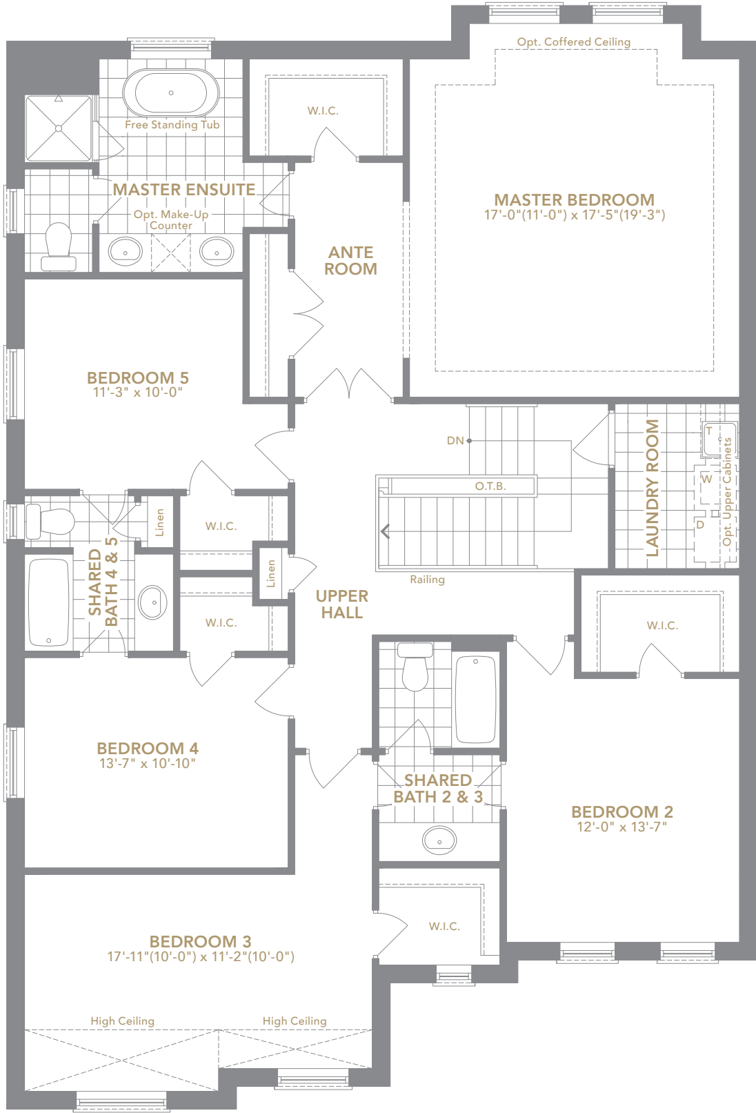
ELEVATION A | SECOND FLOOR | 5 BEDROOM
