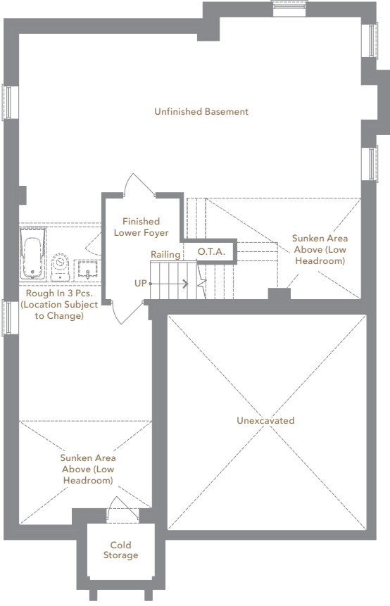
ELEVATION A, B, C BASEMENT
