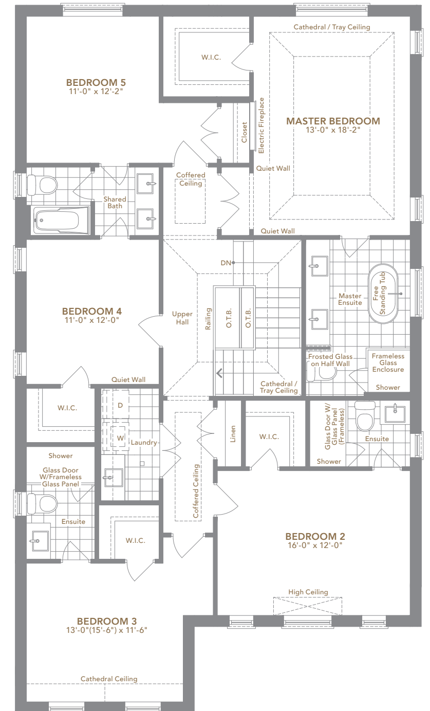
ELEVATION A SECOND FLOOR OPTIONAL 5 BEDROOM
