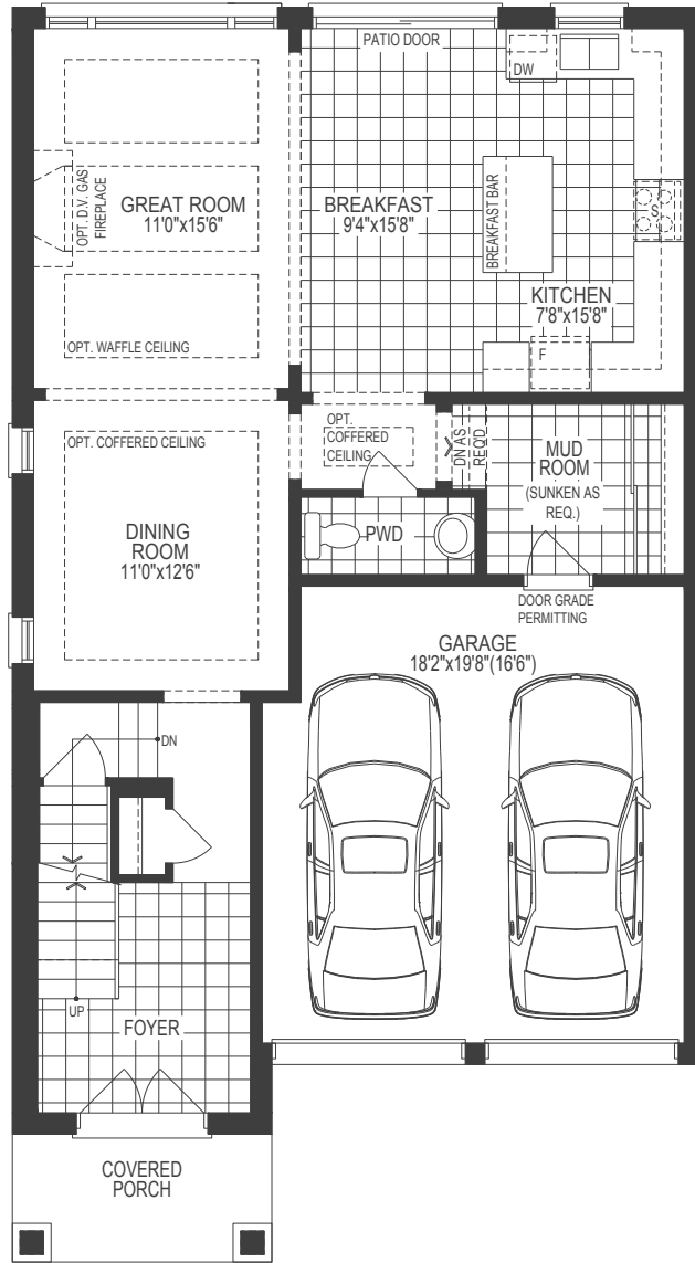
MAIN LEVEL ELEV. B
