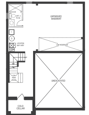
LOWER LEVEL ELEV. B
