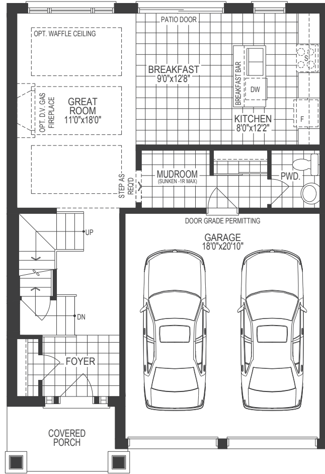
MAIN LEVEL ELEV. B
