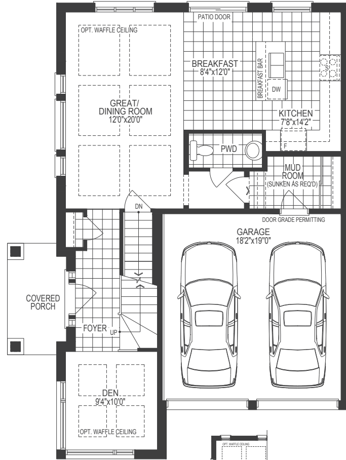
MAIN LEVEL ELEV. B
