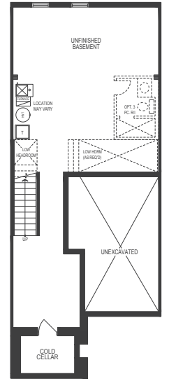
LOWER LEVEL ELEV. A & B
