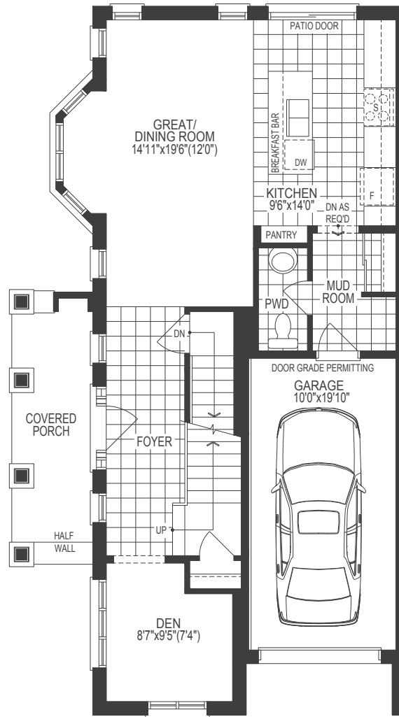
MAIN LEVEL ELEV. A
