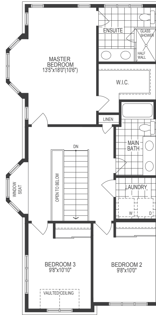
UPPER LEVEL ELEV. A
