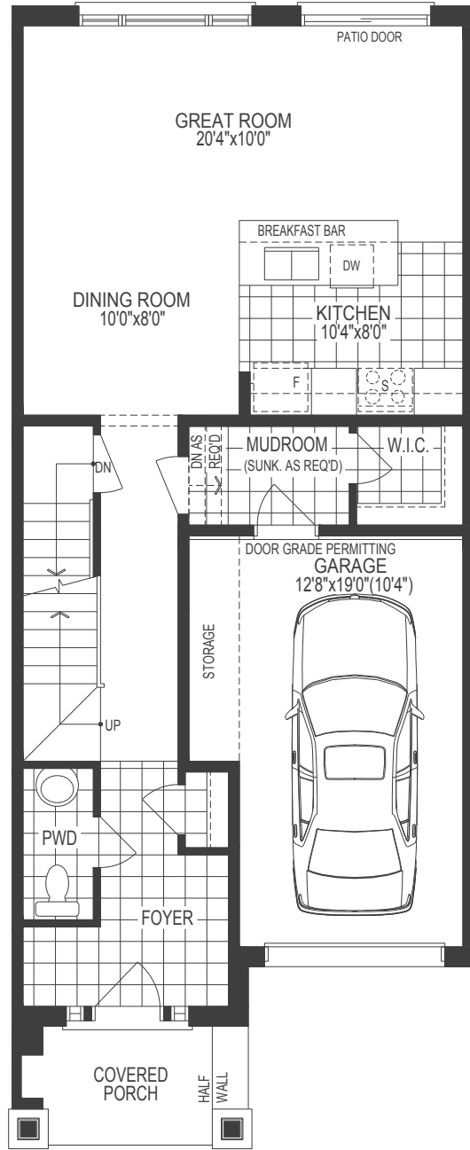
MAIN LEVEL ELEV. A
