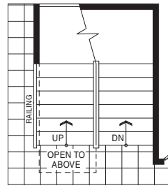
PARTIAL MAIN FLOOR FOR OPTIONAL LOFT STYLE A
