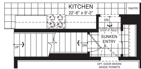
PARTIAL MAIN FLOOR FOR OPTIONAL LOFT STYLE A
