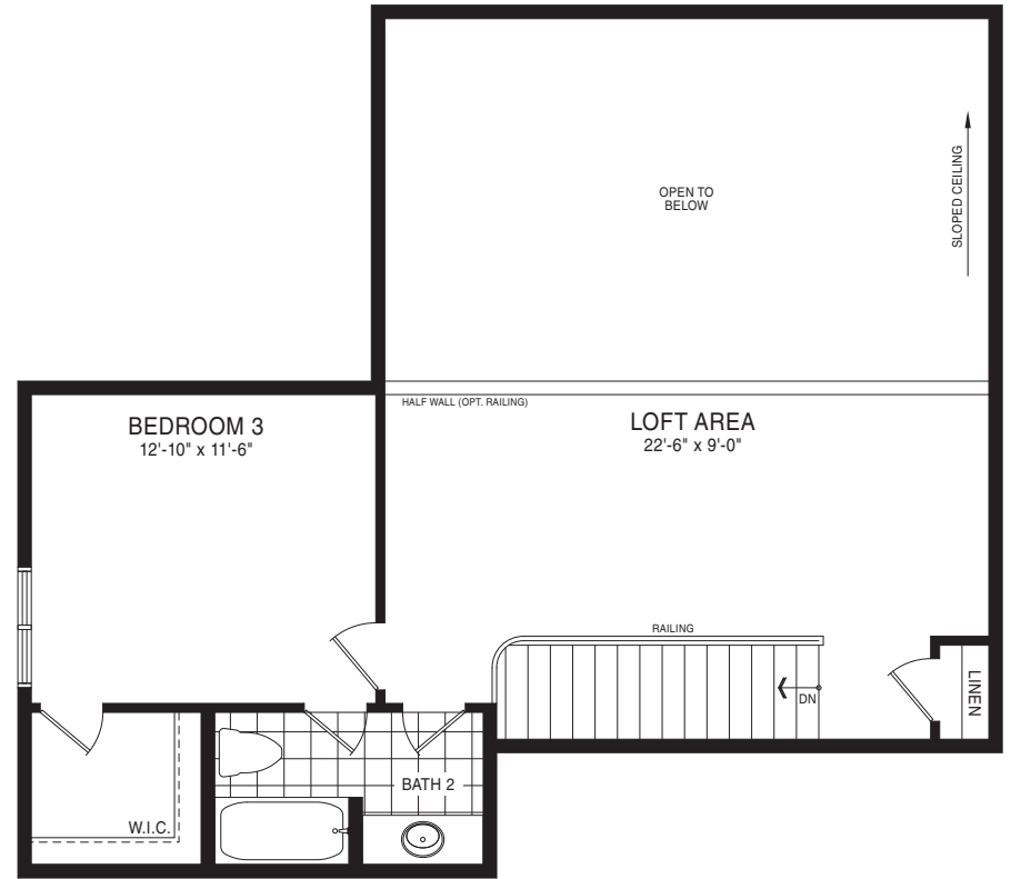
OPTIONAL LOFT PLAN (ALT-L1) STYLE A
