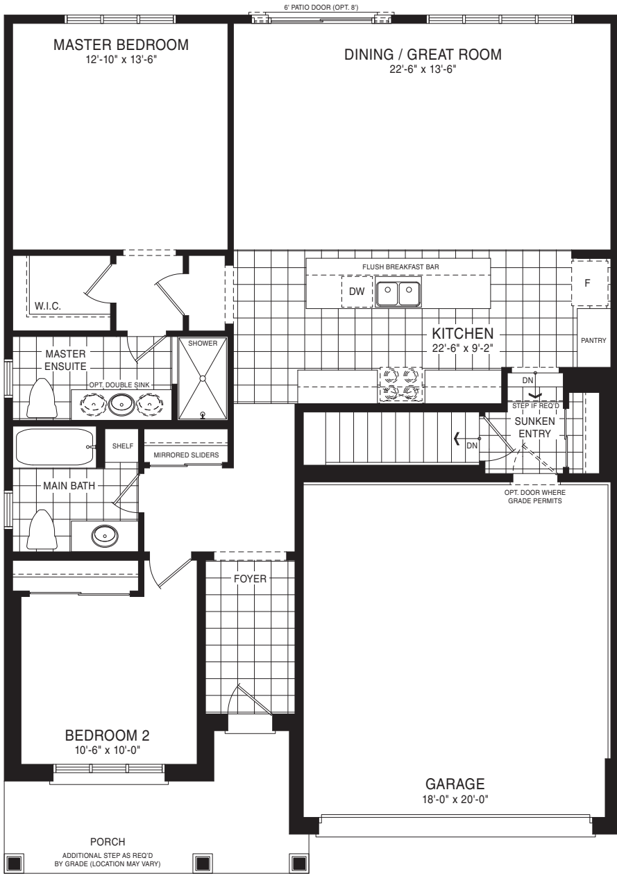
MAIN FLOOR PLAN STYLE A
