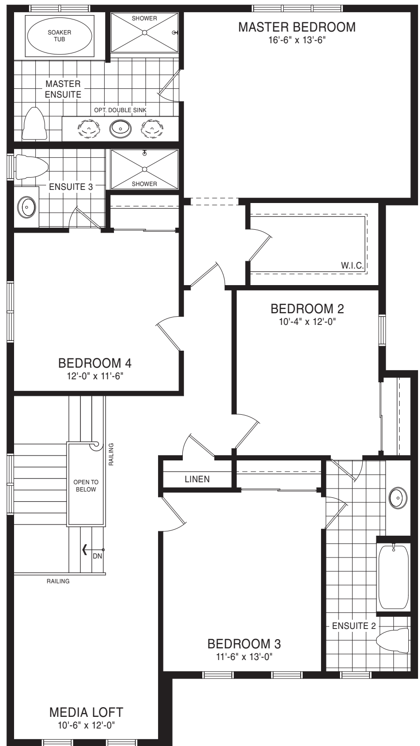
SECOND FLOOR PLAN STYLE A
