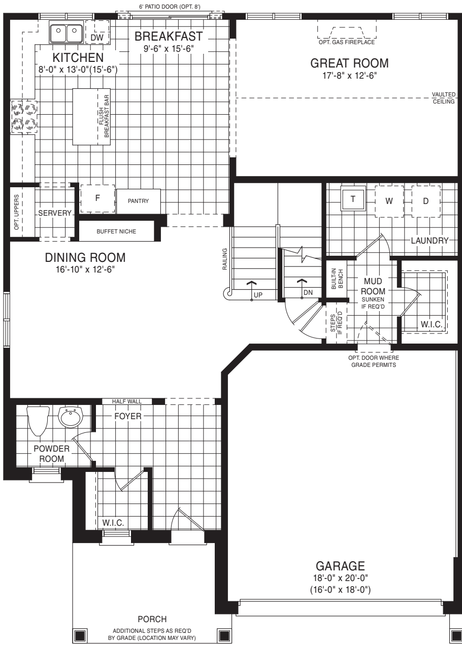
MAIN FLOOR PLAN STYLE A
