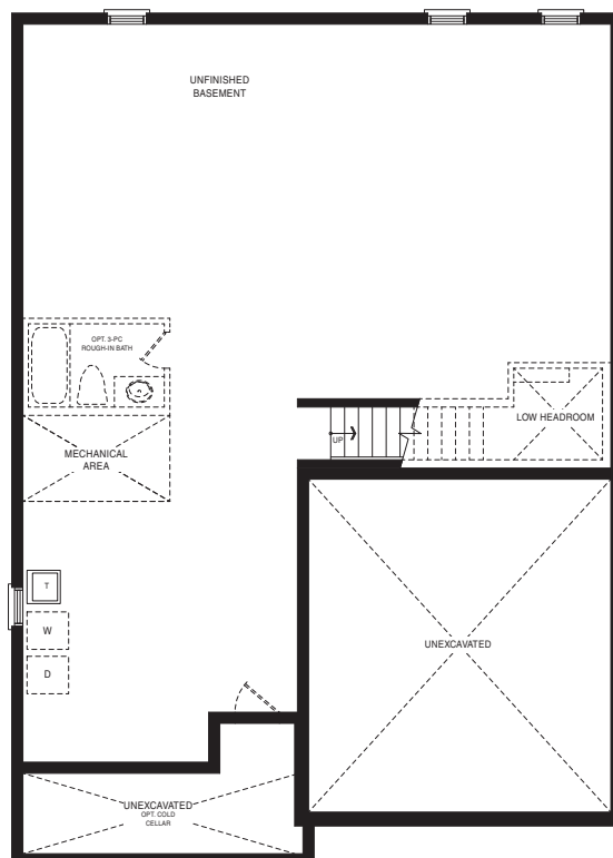
BASEMENT PLAN STYLE A
