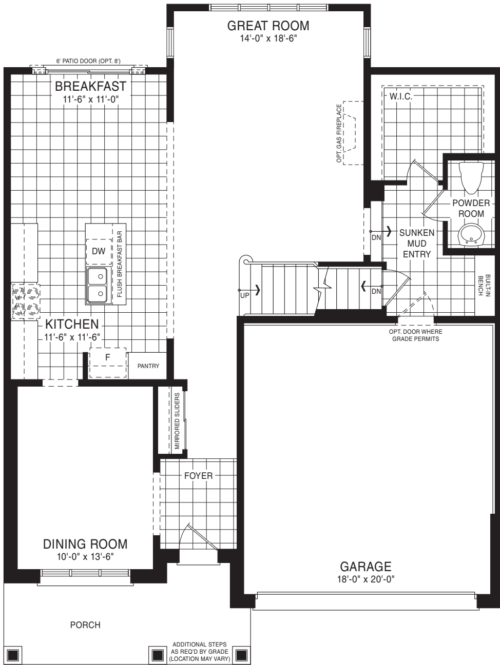
MAIN FLOOR PLAN STYLE A
