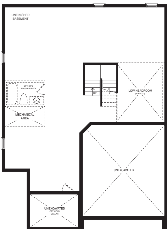
BASEMENT PLAN STYLE A
