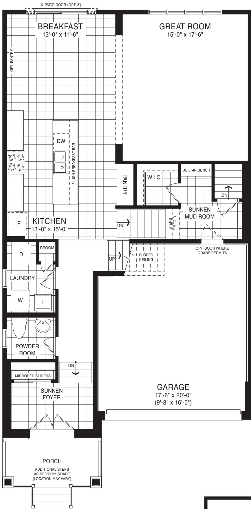
MAIN FLOOR PLAN STYLE A
