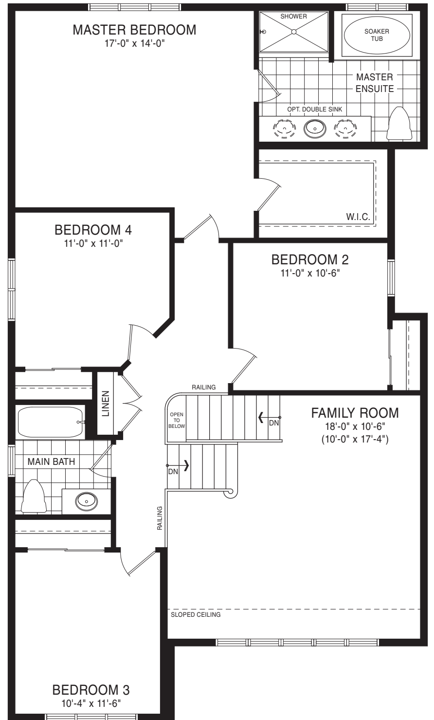
SECOND FLOOR PLAN STYLE A
