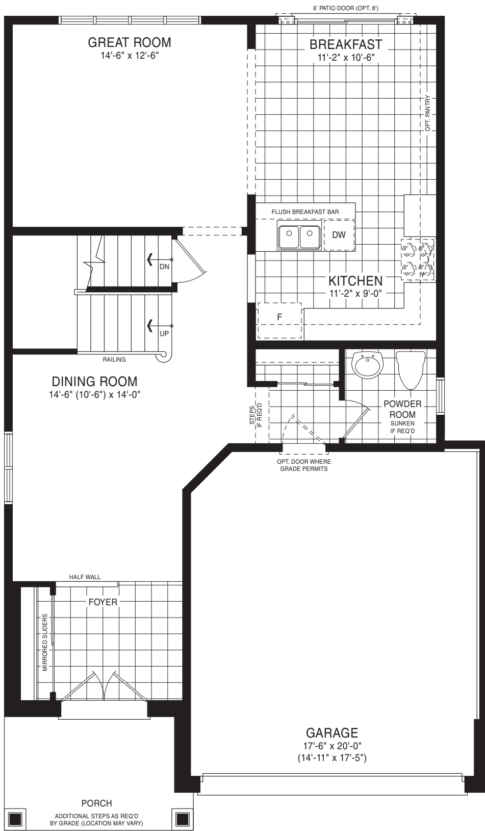
MAIN FLOOR PLAN STYLE A
