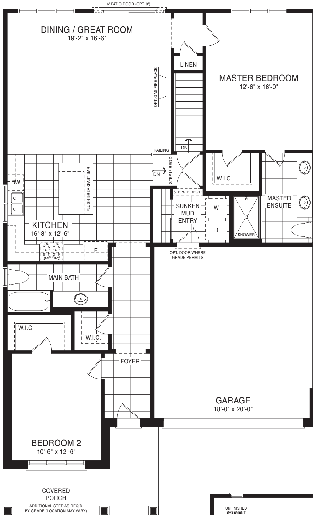
MAIN FLOOR PLAN STYLE A
