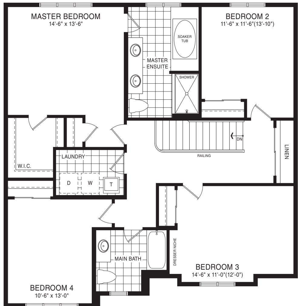
SECOND FLOOR PLAN STYLE A
