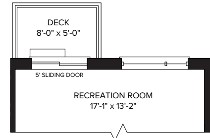
OPT. GROUND FLOOR ELEVATION A & B
