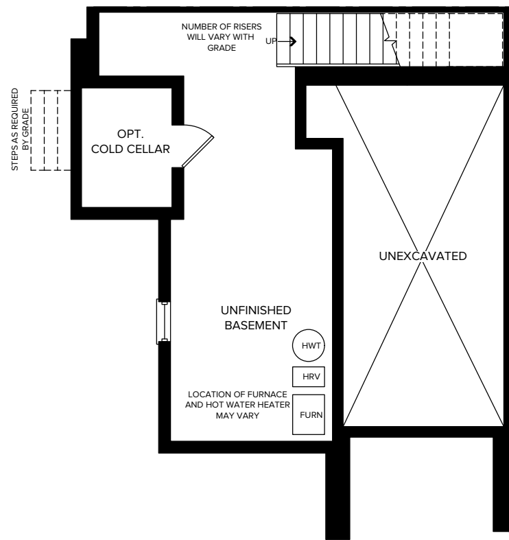
BASEMENT ELEVATION A & B
