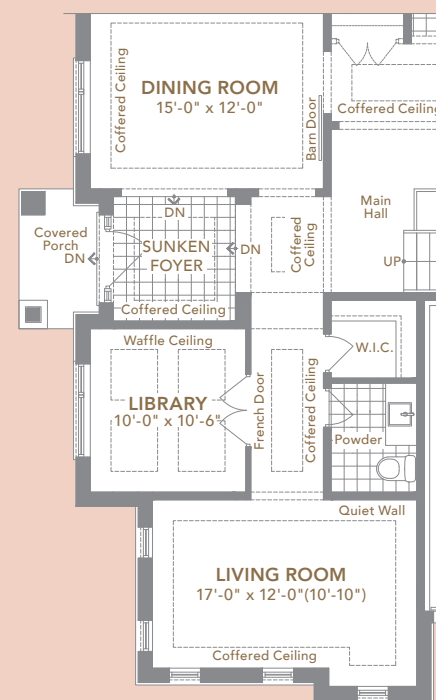
ELEVATION C
