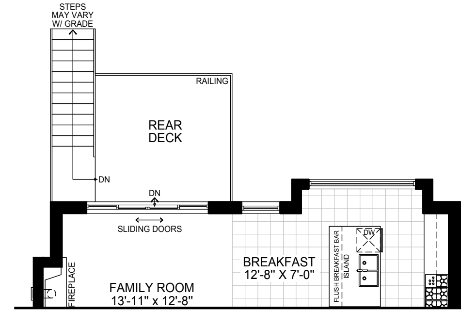
MAIN FLOOR ELEVATION C
