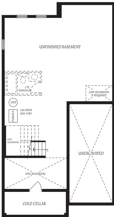
BASEMENT ELEVATION A
