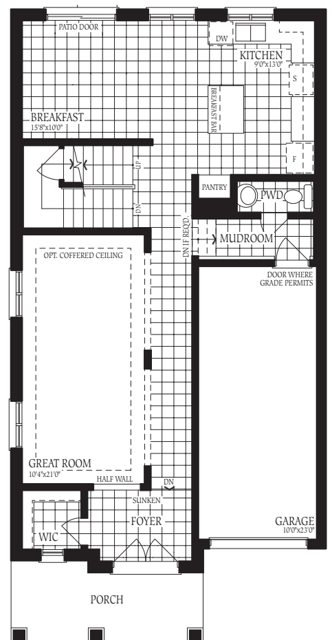
ALT. GROUND FLOOR ELEVATION A
