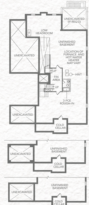
ELEVATION A, B, C BASEMENT
