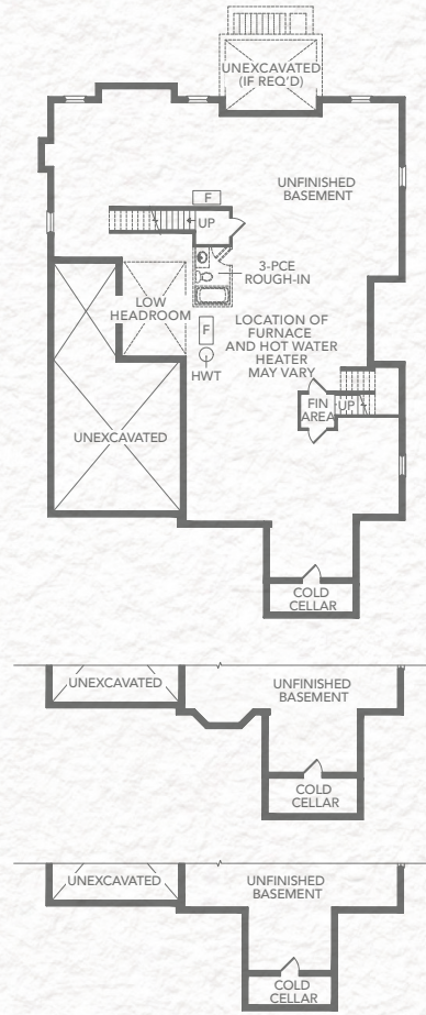
ELEVATION A, B, C BASEMENT
