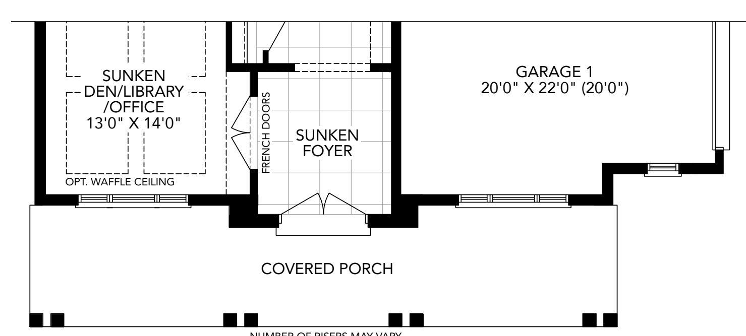
OPTIONAL GROUND FLOOR PLAN FOR COACH HOUSE ELEVATION A
