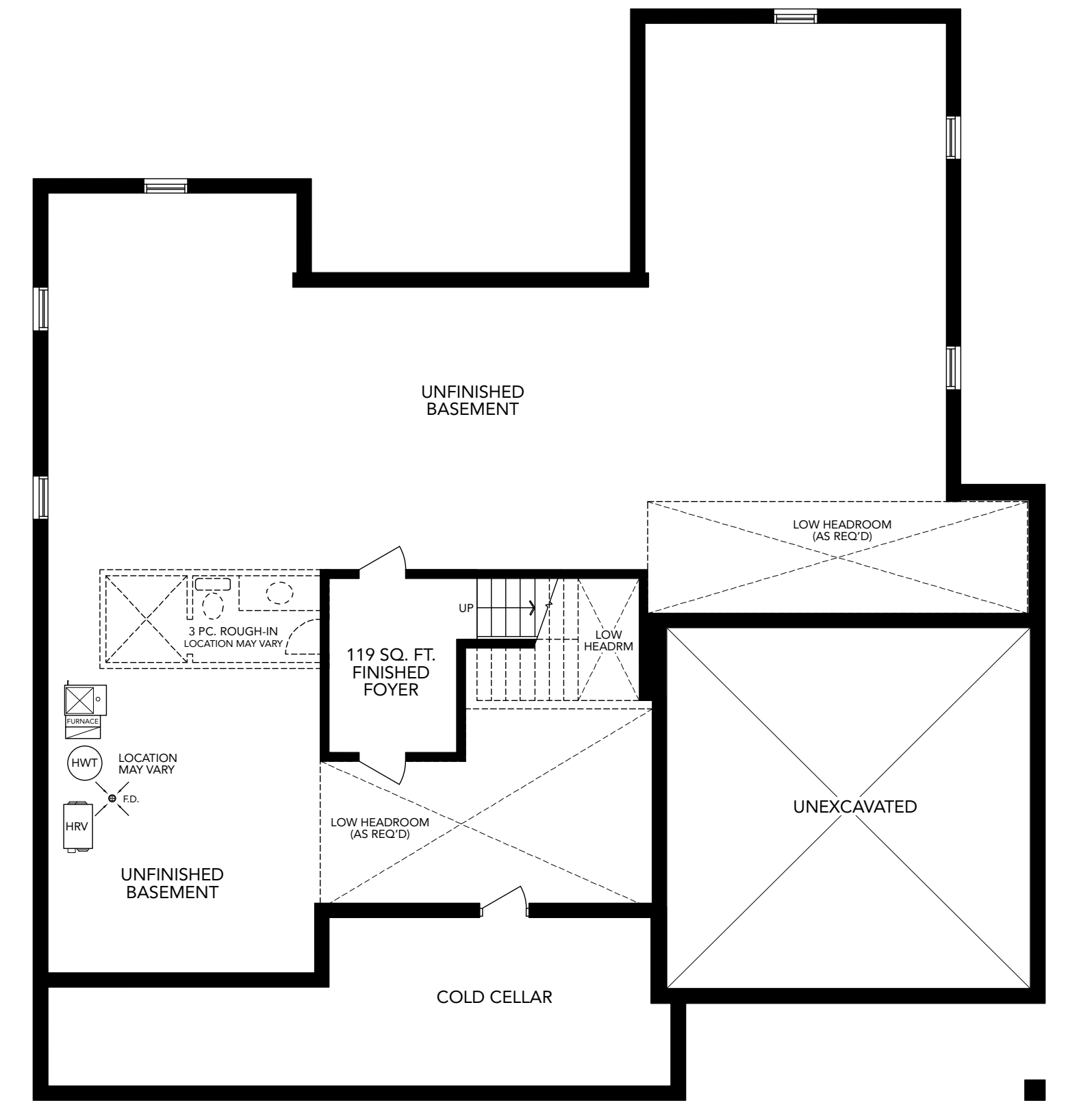
BASEMENT FLOOR PLAN ELEVATION A
