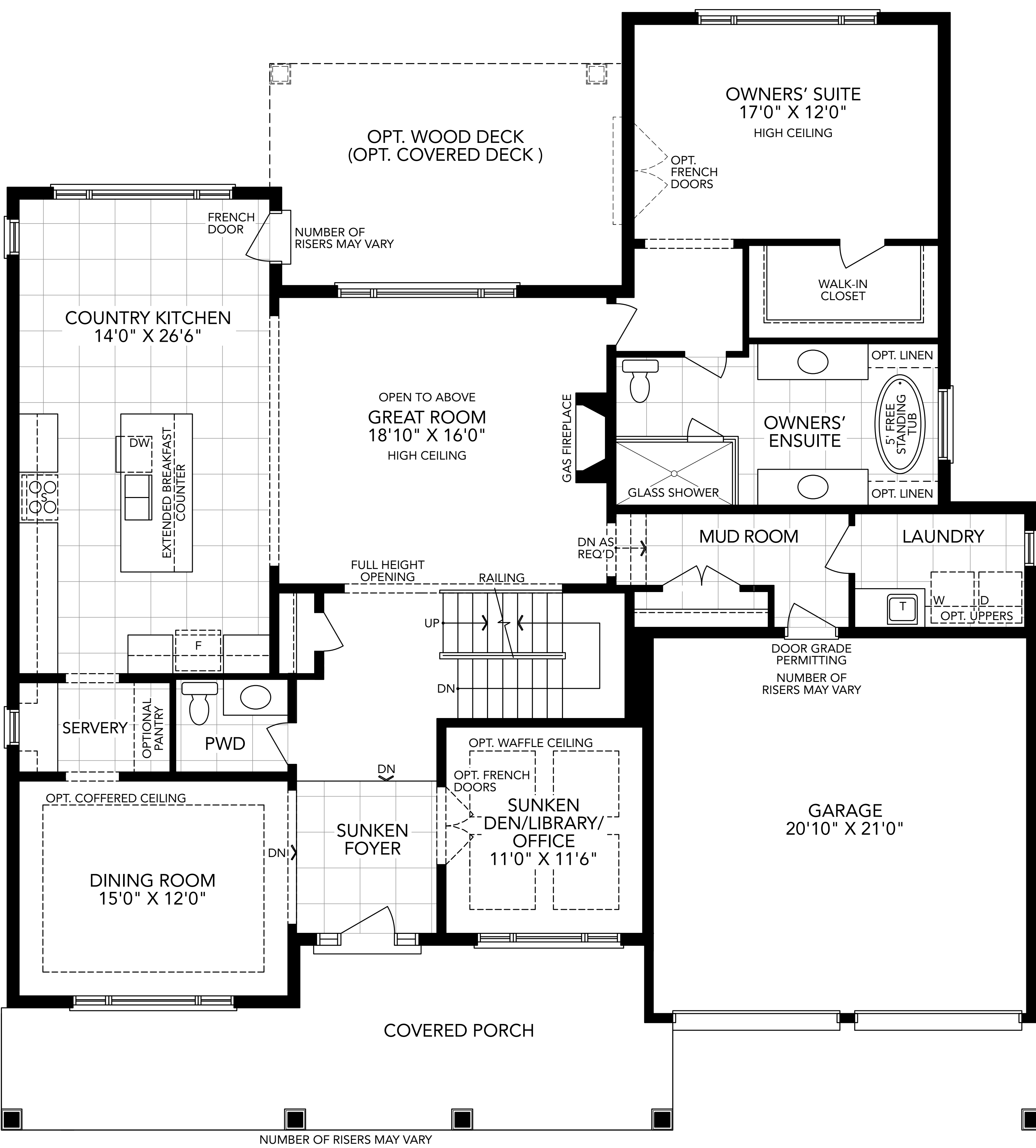
GROUND FLOOR PLAN ELEVATION A
