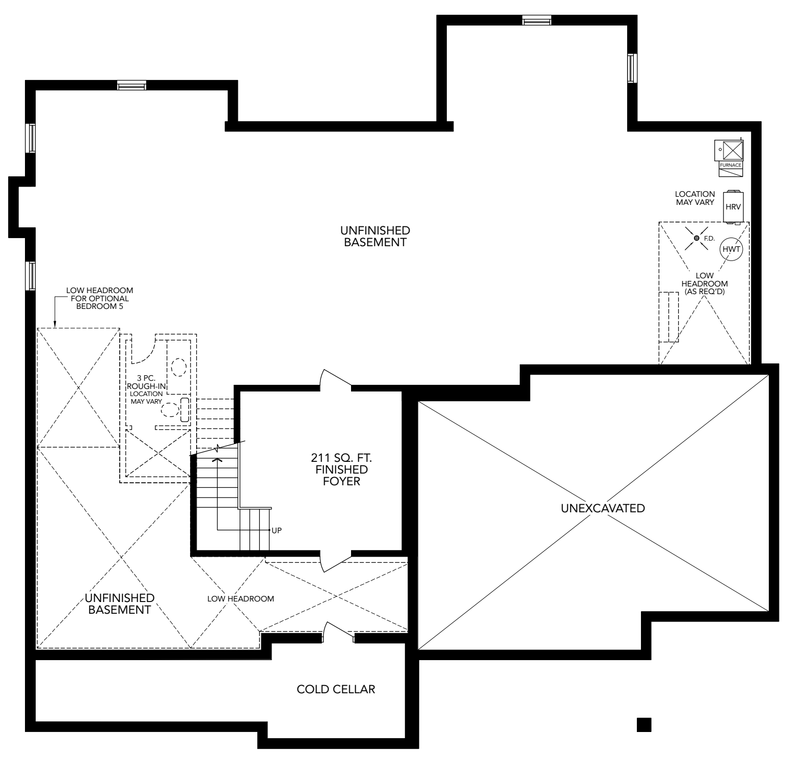
BASEMENT FLOOR PLAN ELEVATION A
