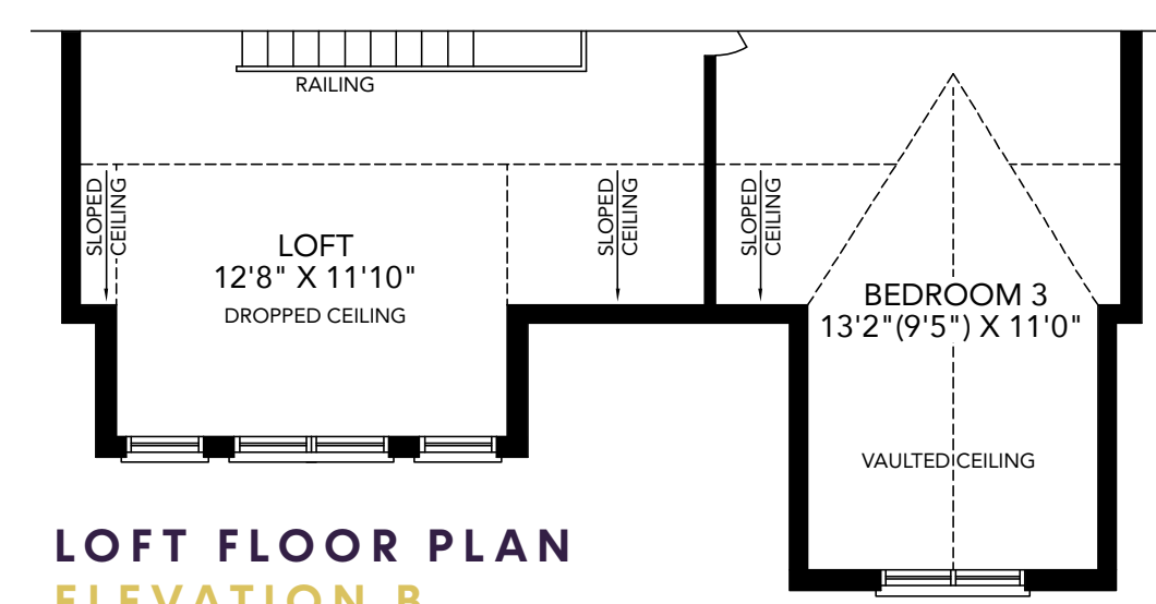
LOFT FLOOR PLAN ELEVATION B
