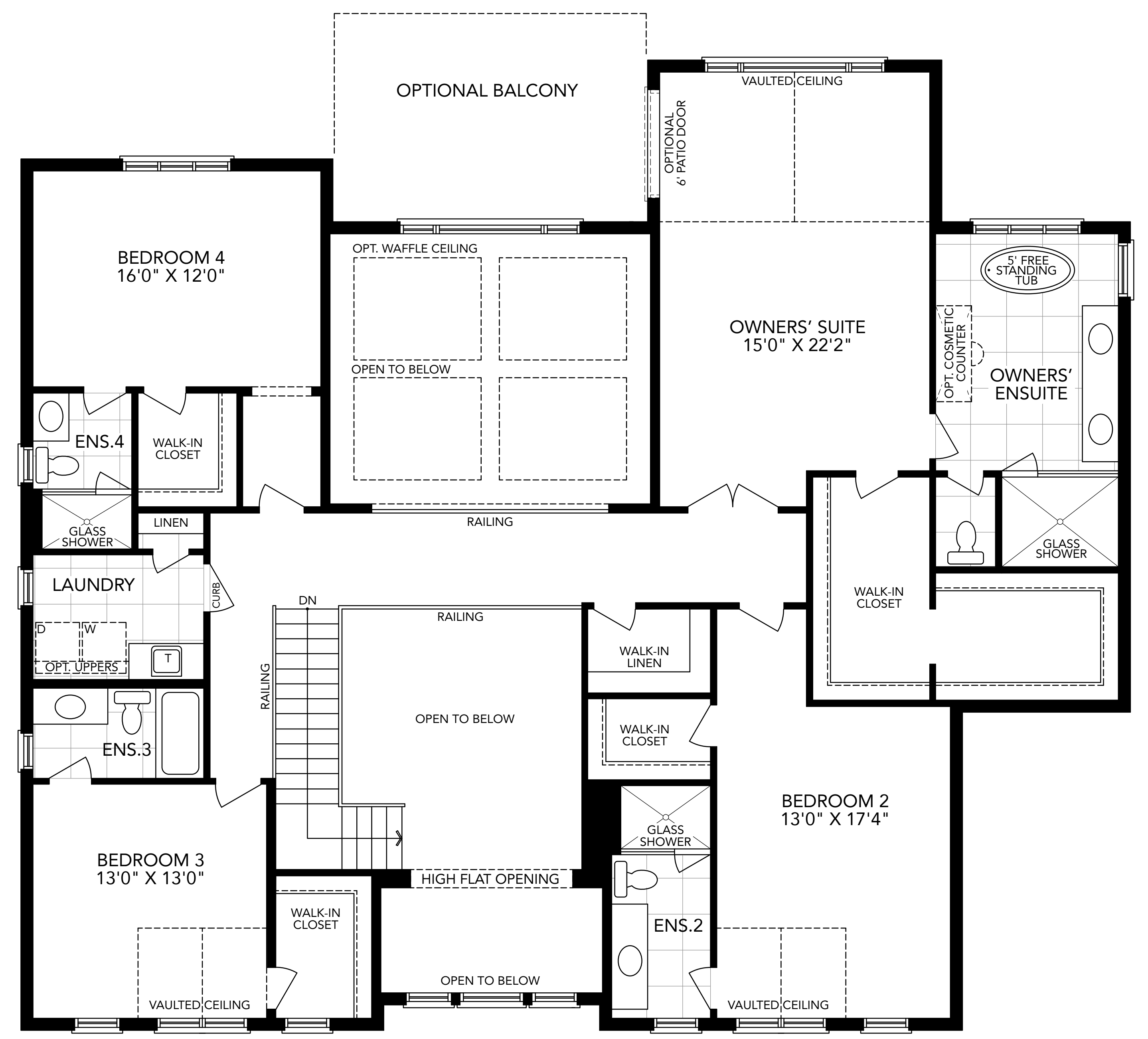
SECOND FLOOR PLAN ELEVATION A
