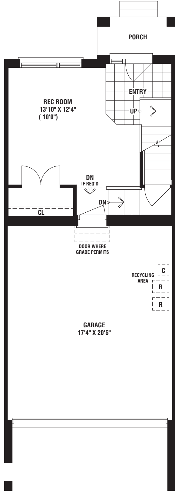
GROUND FLOOR ELEVATION 'A1'
