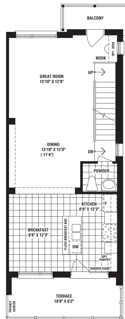
SECOND FLOOR ELEVATION 'A3' INTERIOR END
