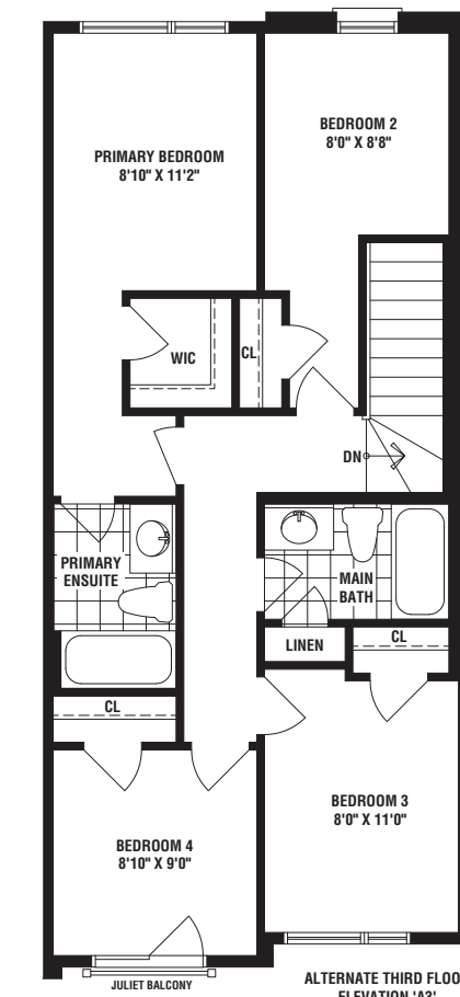
ALTERNATE THIRD FLOOR ELEVATION 'A3' INTERIOR END
