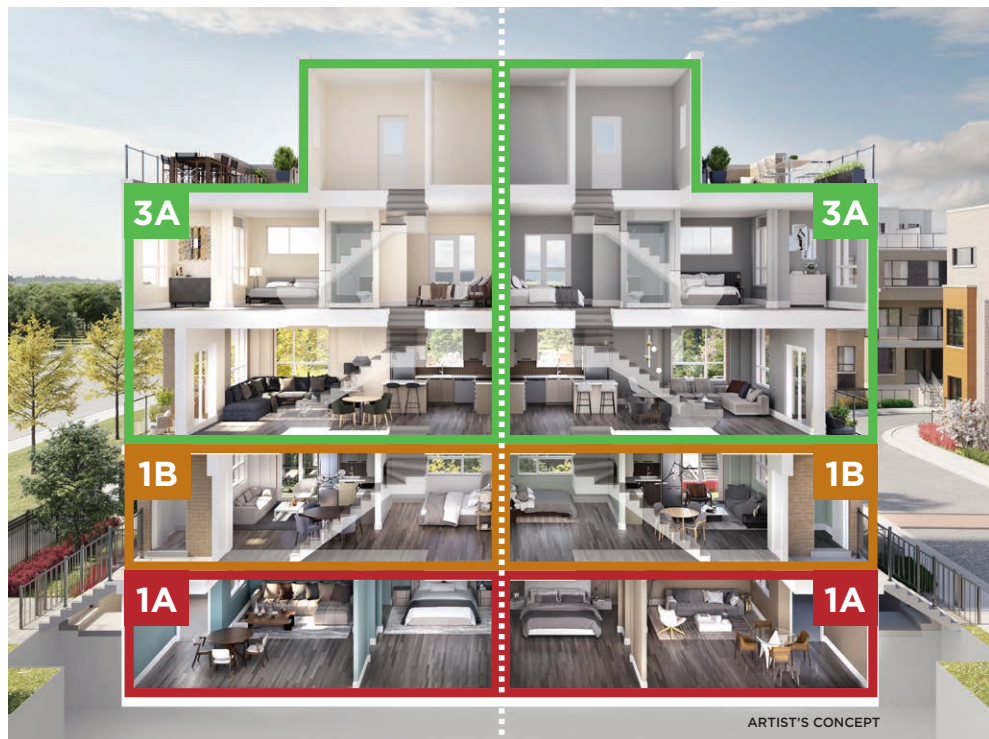
CROSS SECTION A
