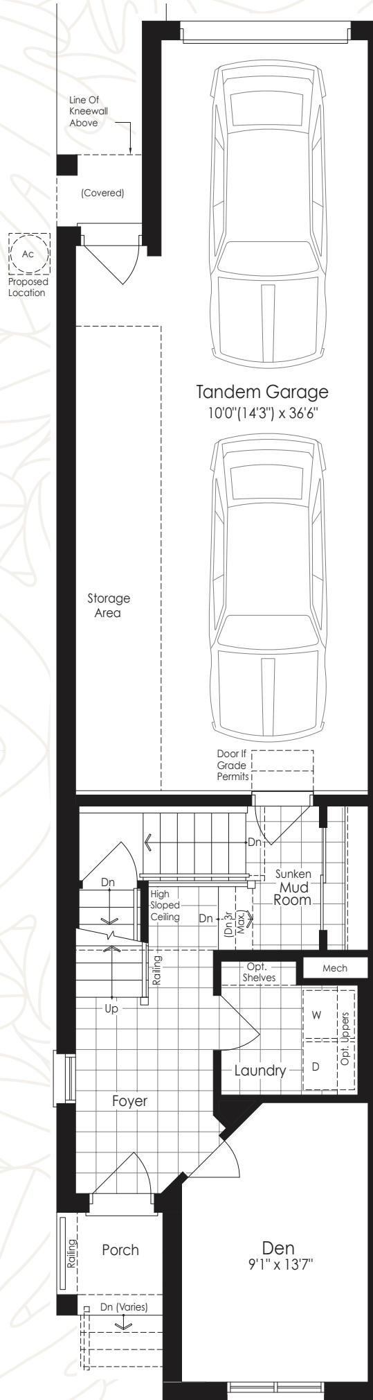
Ground Floor Elev. A
