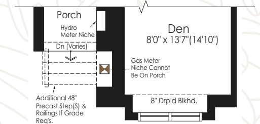
Ground Floor Elev. B
