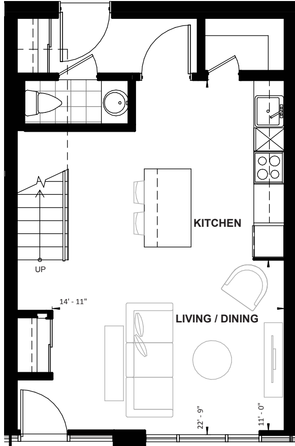
TH LEVEL 01
