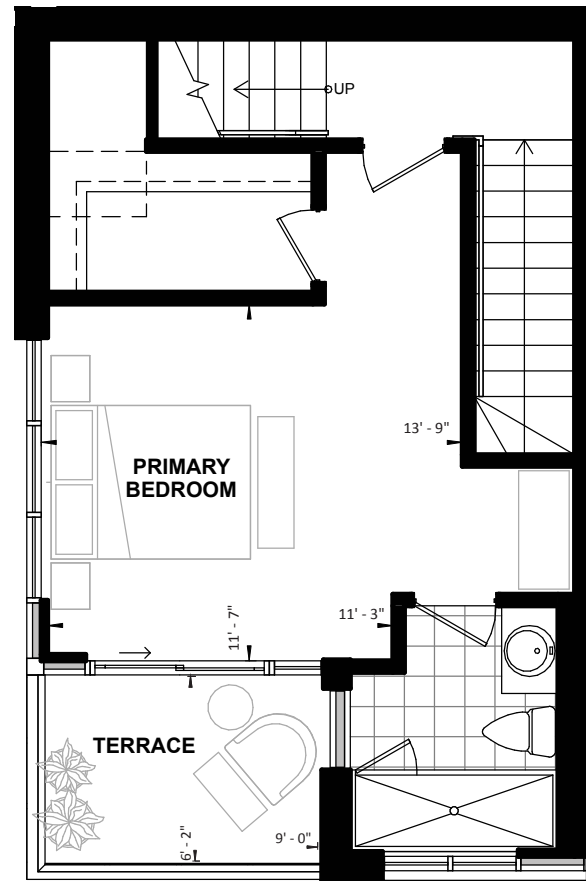
TH LEVEL 03
