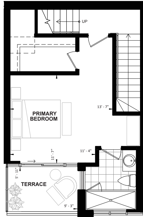
TH LEVEL 03
