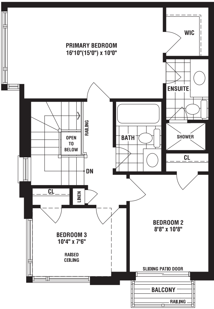
UPPER FLOOR PLAN ELEV. 'B'
