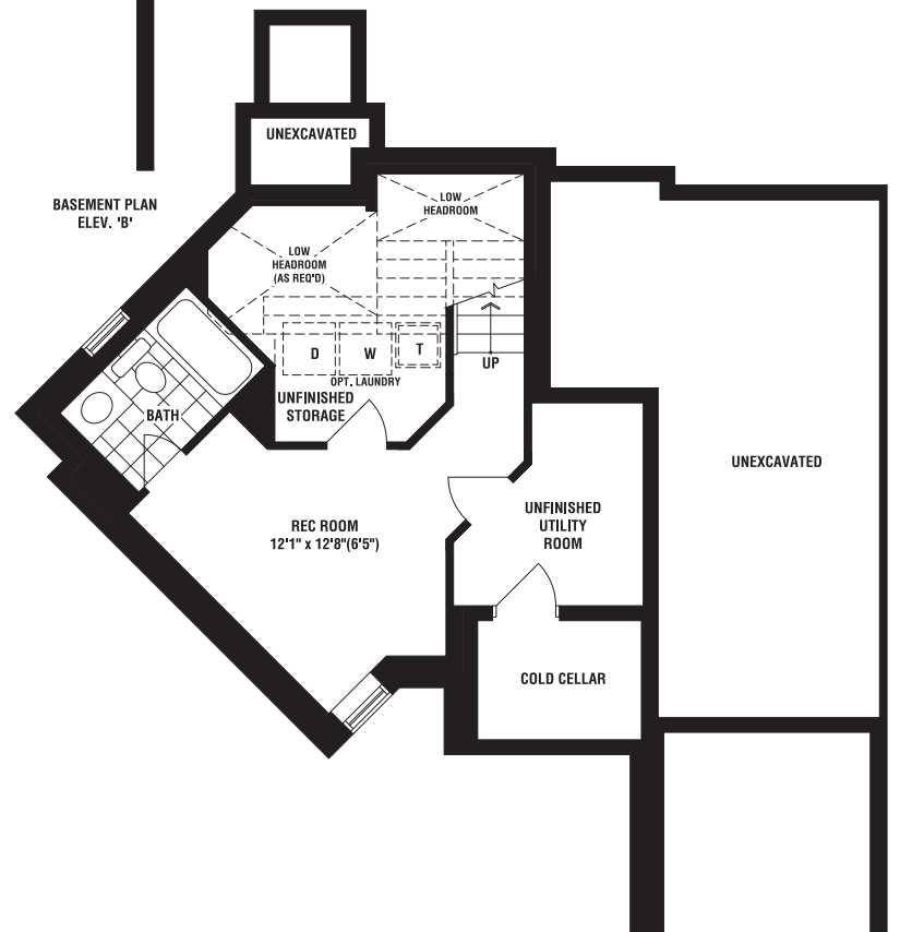
OPT. FINISHED BASEMENT PLAN ELEV. 'B' (Not including 381 sq.ft. finished basement)
