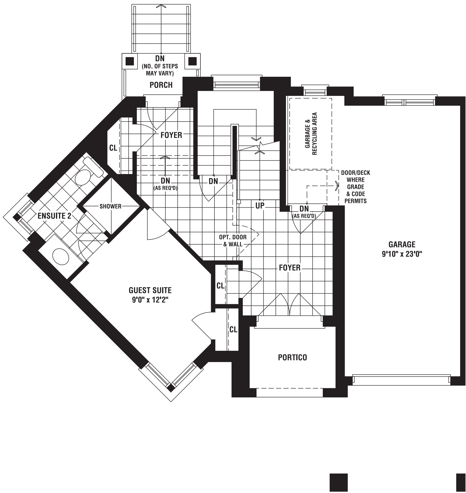
GROUND FLOOR PLAN ELEV. 'B'
