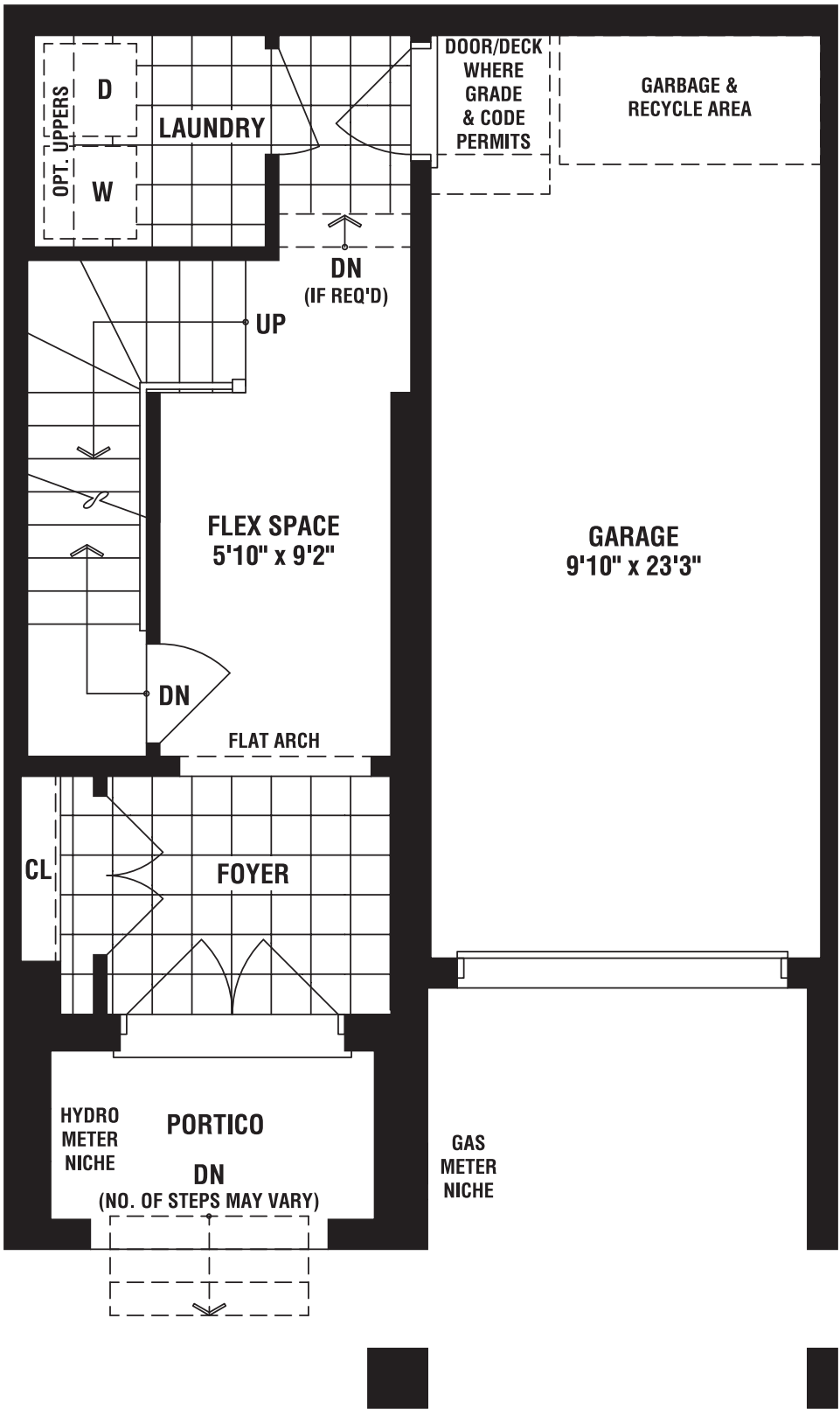
GROUND FLOOR PLAN ELEV. 'A'
