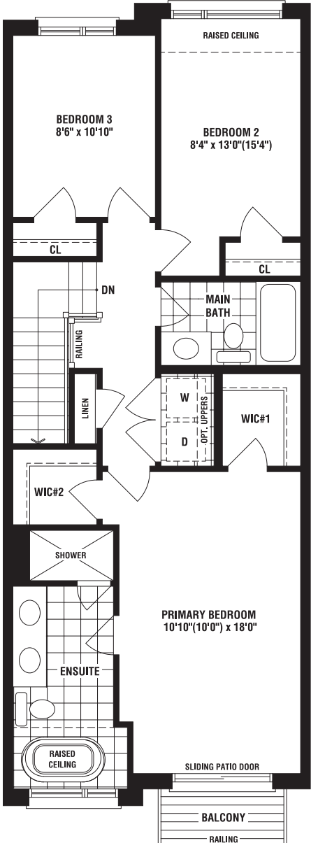
UPPER FLOOR PLAN ELEV. 'B'
