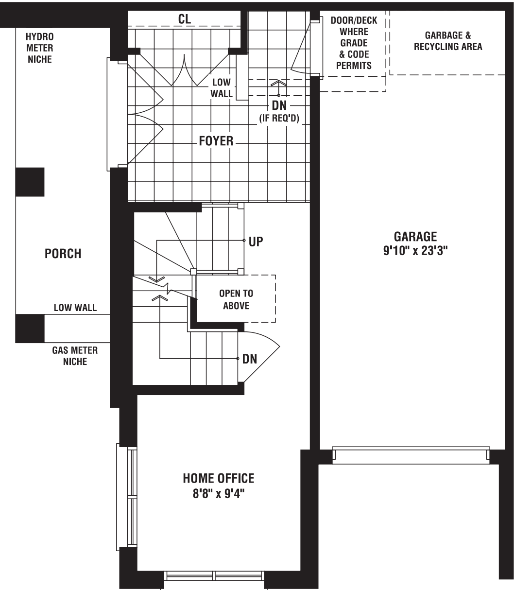
GROUND FLOOR PLAN ELEV. 'A'
