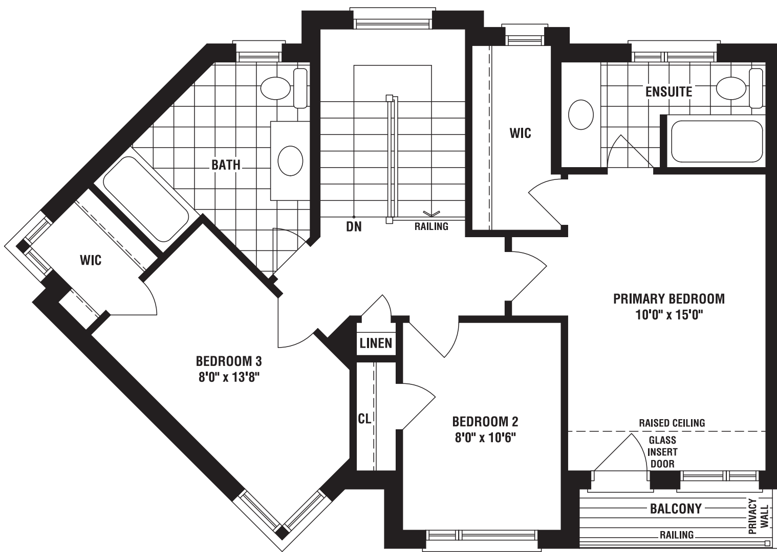
UPPER FLOOR PLAN ELEV. 'B'
