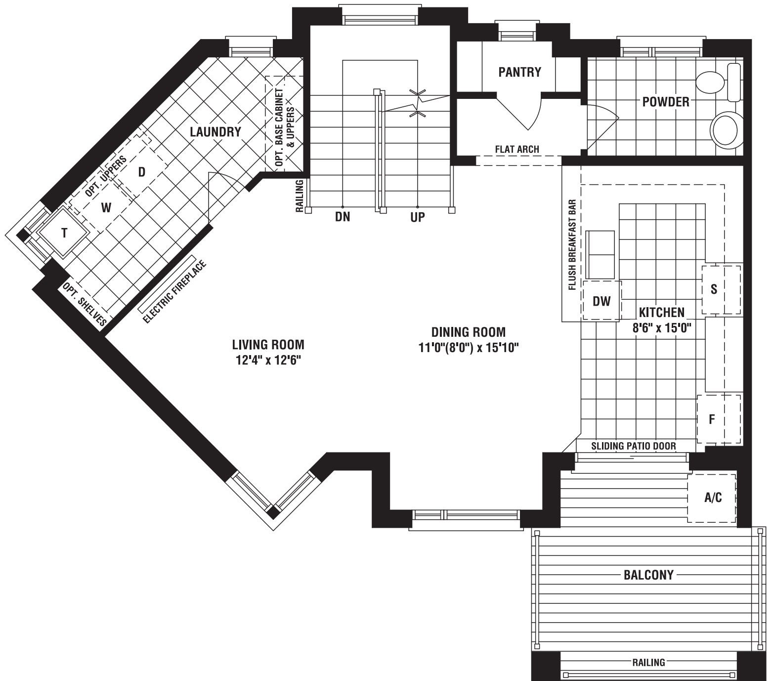
MAIN FLOOR PLAN ELEV. 'B'
