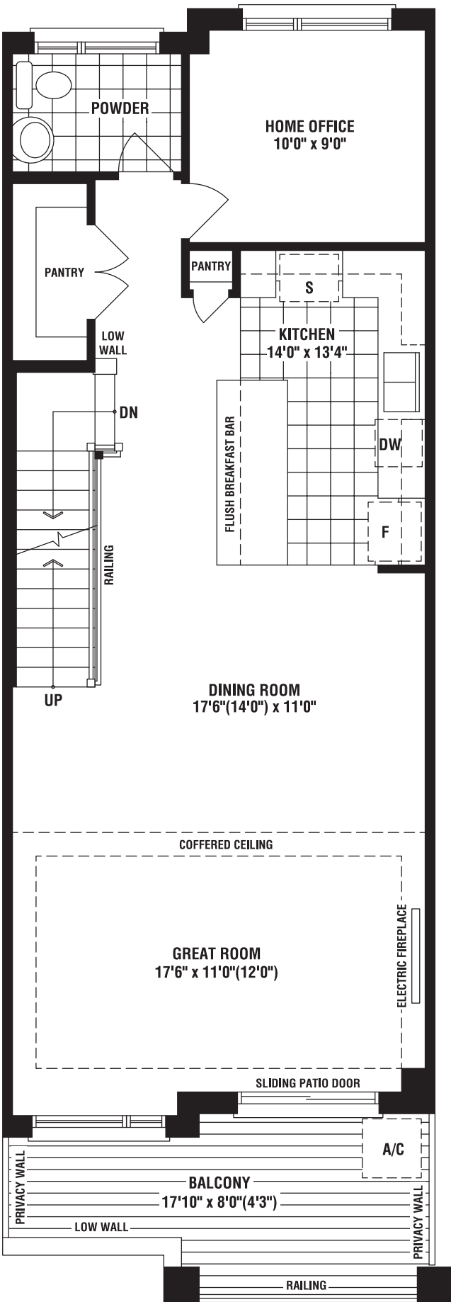
MAIN FLOOR PLAN ELEV. 'A'
