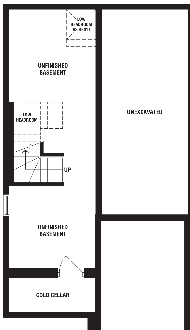
BASEMENT PLAN ELEV. 'B'
