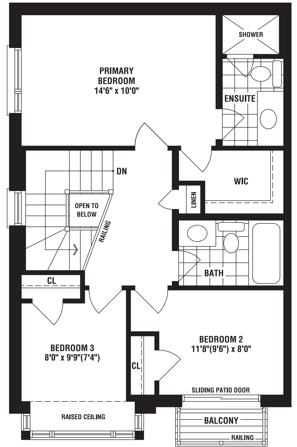
UPPER FLOOR PLAN ELEV. 'B'
