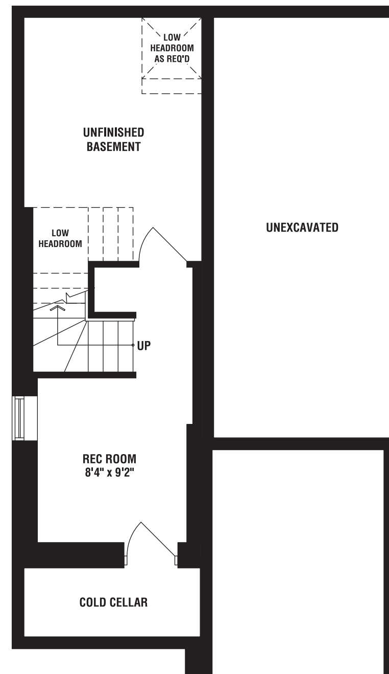
OPT. FINISHED BASEMENT PLAN ELEV. 'B' (Not including 151 sq.ft. finished basement)
