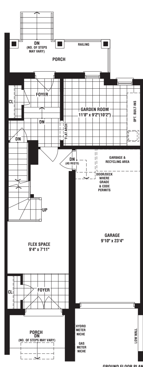
GROUND FLOOR PLAN ELEV. 'B2'
