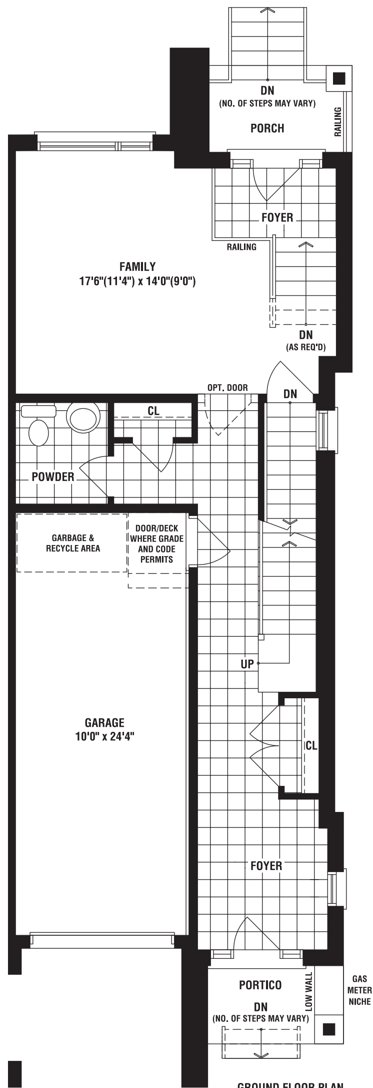
GROUND FLOOR PLAN ELEV. 'B' BLOCK 5, UNIT 26
