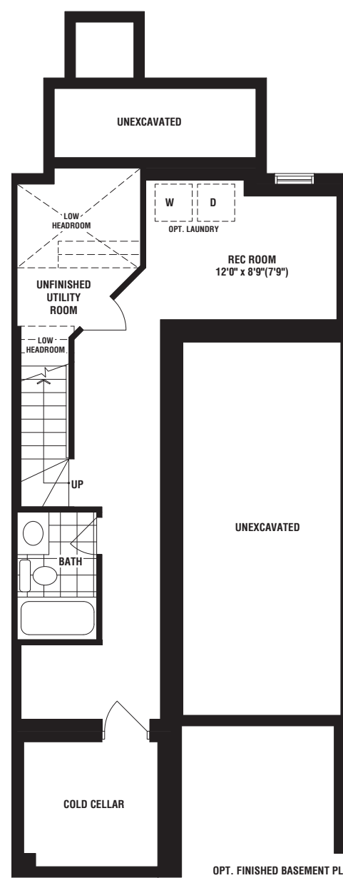
OPT. FINISHED BASEMENT PLAN ELEV. 'B1'/'B1Mod' (Not including 352 sq.ft. finished basement)
