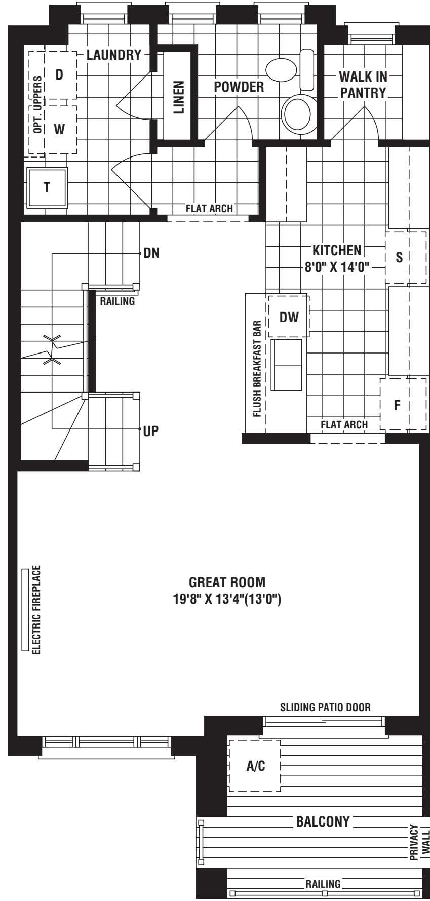
MAIN FLOOR PLAN ELEV. 'B1'/'B1Mod'
