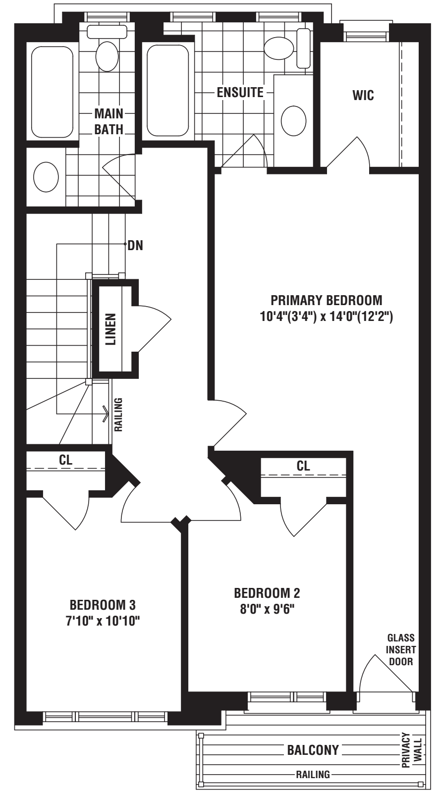
UPPER FLOOR PLAN ELEV. 'B1'/'B1Mod'
