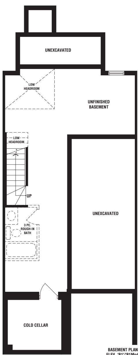
BASEMENT PLAN ELEV. 'B1'/'B1Mod'
