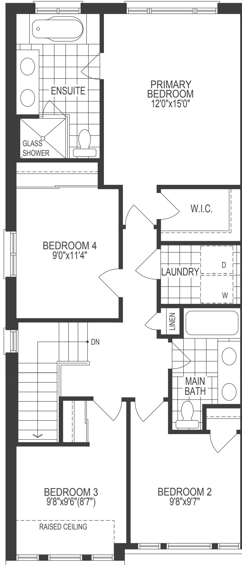
UPPER LEVEL ELEV. B
