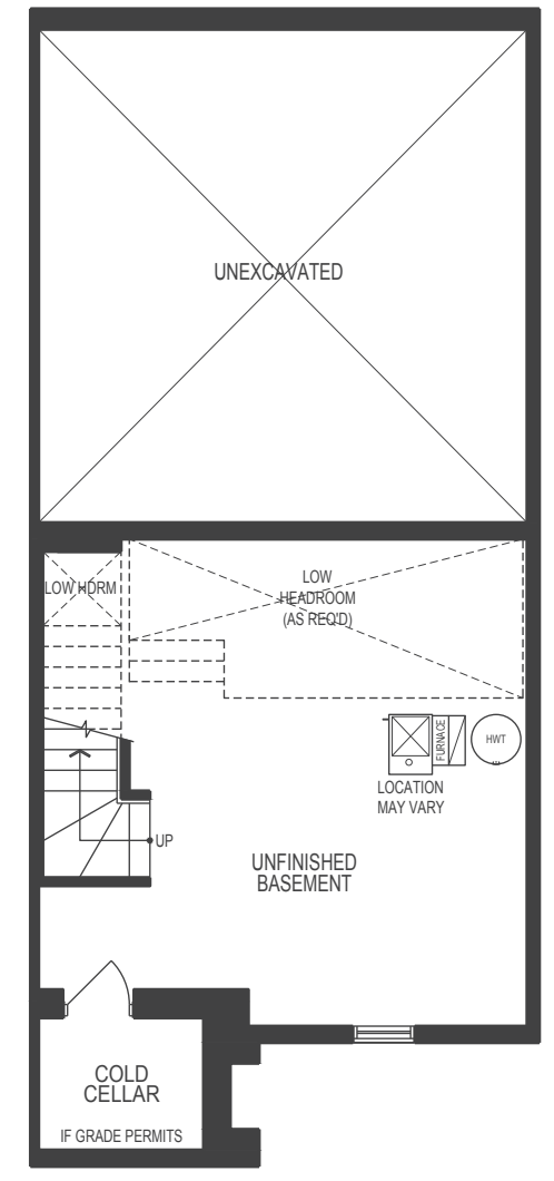
LOWER LEVEL B
