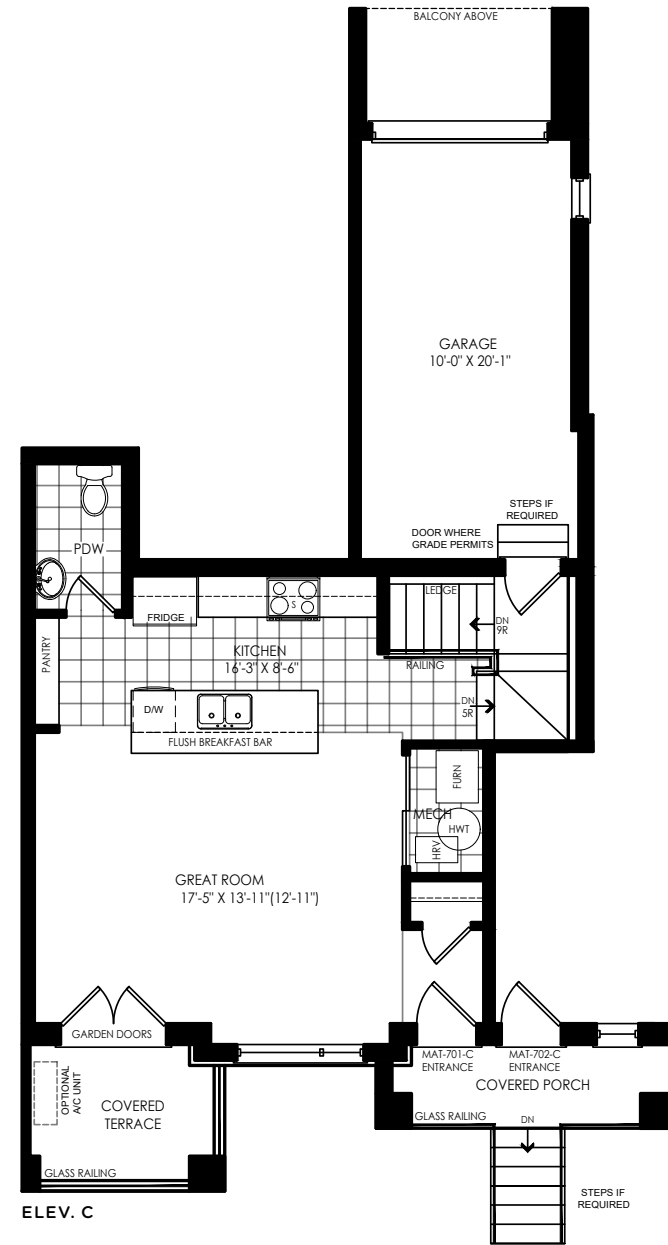
FIRST LEVEL
