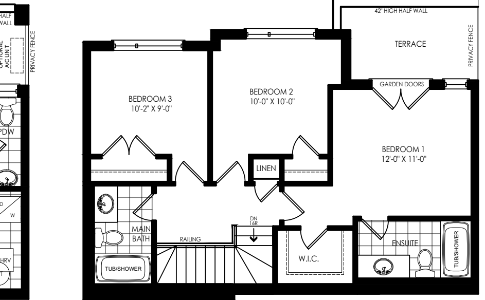
THIRD LEVEL
